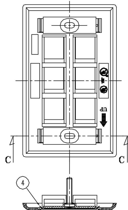
Section: C-C
